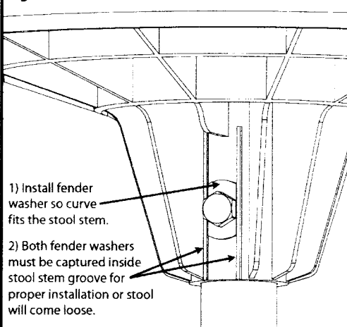
Figure #3: CRITICAL ASSEMBLY DETAIL
